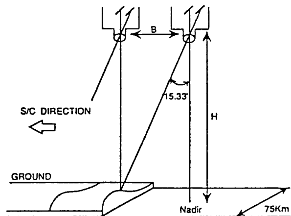
Figure 1. Imaging geometry of the JERS-1 VNIR instrument (reproduced from NASDA, 1990).
