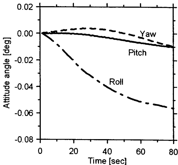
Figure 3. Attitude variation in the strip.
