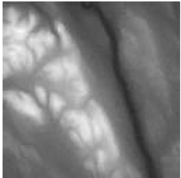
Figure 9. DEM computed in test case 1.
